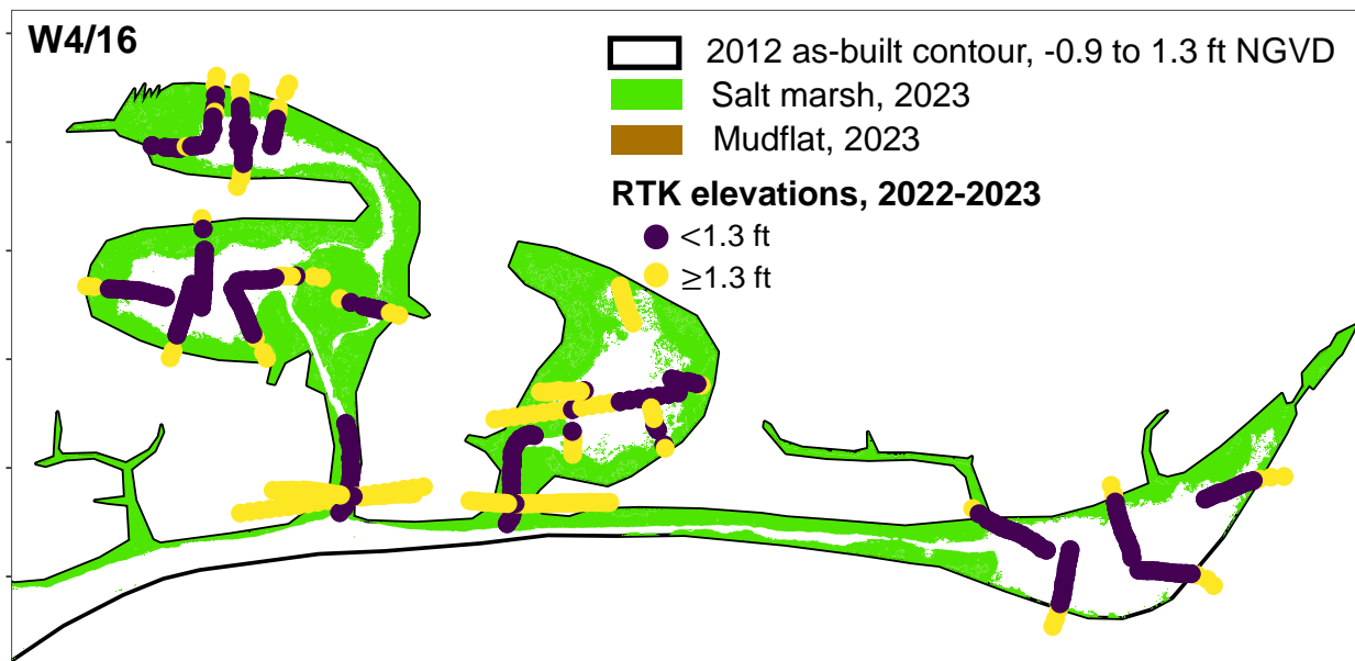
Figure 7.2.7. RTK elevation surveys within planned mudflat habitat (black line; 1.3' NGVD contour). Yellow dots indicate elevations greater than 1.3' NGVD; dark purple points indicate elevations less than 1.3' NGVD.
