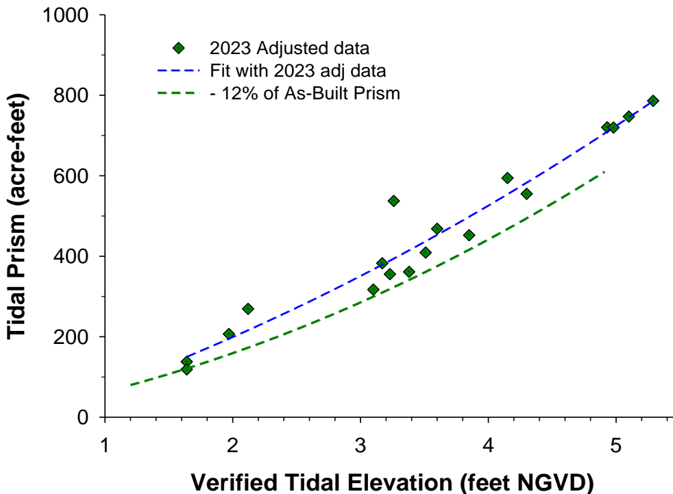
Figure 5.1.1.2. The regression fit to the tidal prism measurements taken January-December 2023 (blue dashed line) must fall above the green line, which represents 88% of the as-built prism, for the tidal prism to be maintained. Tidal prism measurements for 2023 were adjusted for the excavation of additional wetland by the 22 nd Agricultural District adjacent to the Grand Avenue Bridge.
