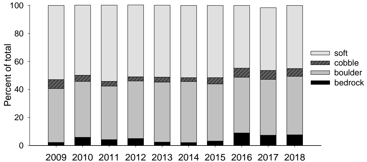
Figure 5.1.3. Distribution of substrate types on Wheeler North Reef from 2009 – 2018.
