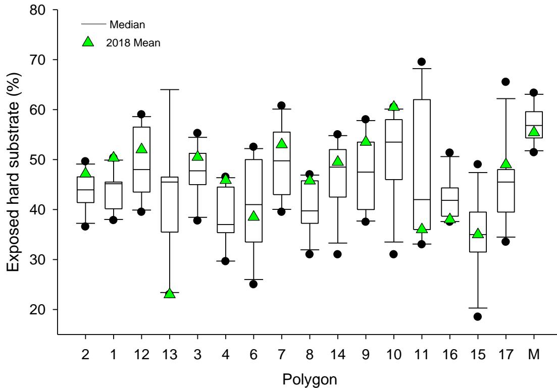
Figure 5.1.2. Mean percent cover of exposed hard substrate in the Phase 2 polygons of Wheeler North Reef from 2009 – 2018. Box boundaries indicate the 25 th and 75 th percentiles and the whiskers are the 10 th and 90 th percentile. Solid points represent the upper and lower range. Polygon numbers are ordered from south to north. M represents the 12 Phase 1 modules.
