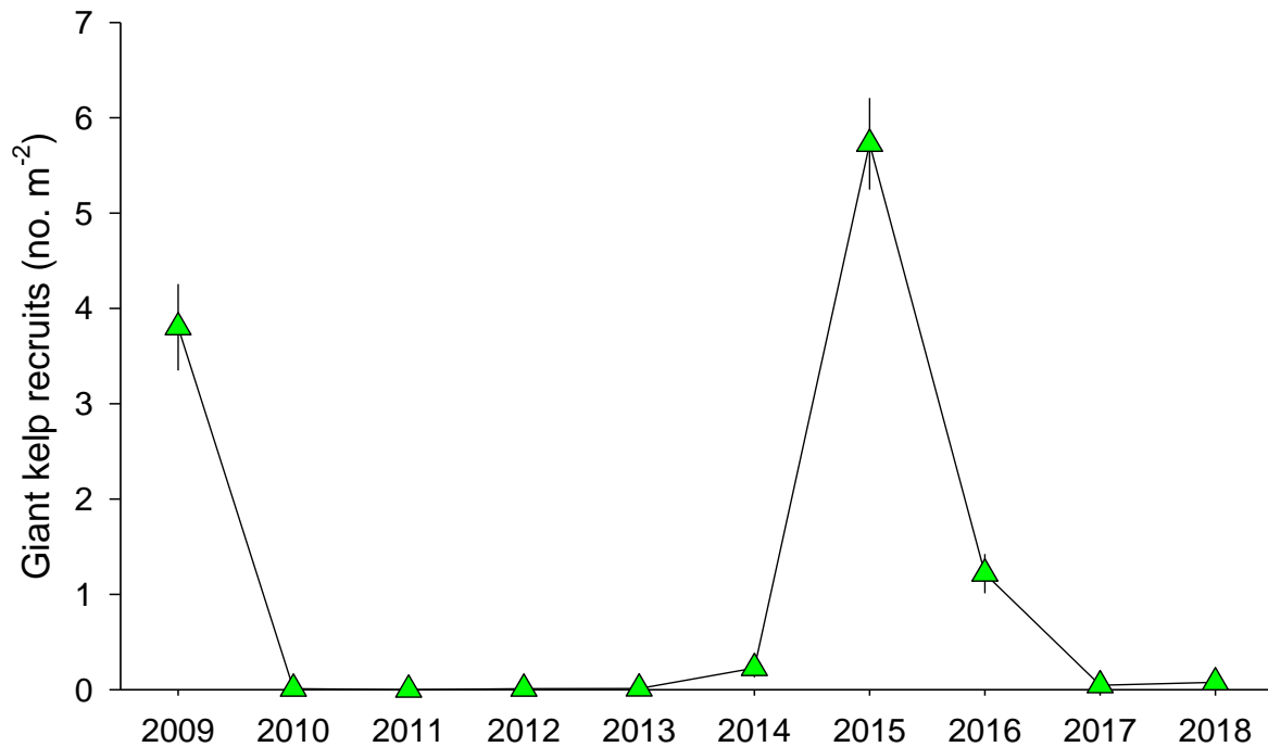
Figure 5.2.1. Mean density ( \pm 1 standard error) of newly recruited giant kelp plants ( Macrocystis pyrifera ) at Wheeler North Reef from 2009 – 2018.
