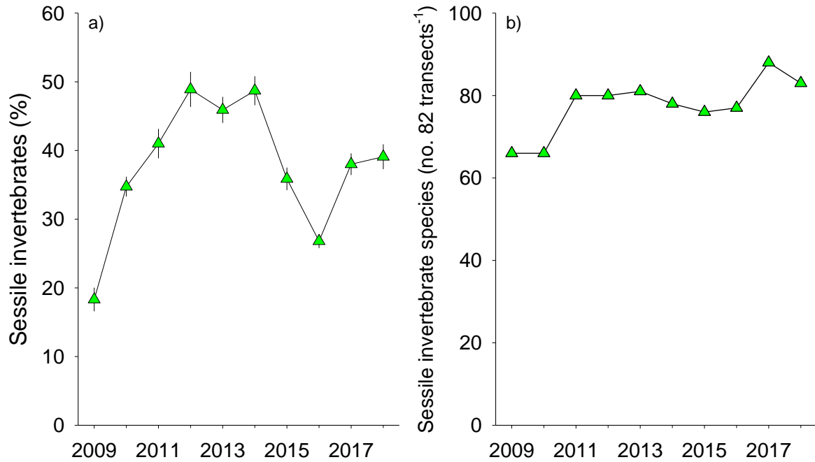
Figure 5.2.11. (a) Mean percent cover ( \pm 1 standard error) and (b) total number of species of sessile invertebrates at Wheeler North from 2009 – 2018.
