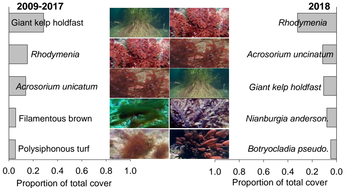
Figure 5.2.10. Proportion of the total percent cover of algae contributed by the five most abundant algal species at Wheeler North Reef averaged for 2009 – 2017 and 2018.
