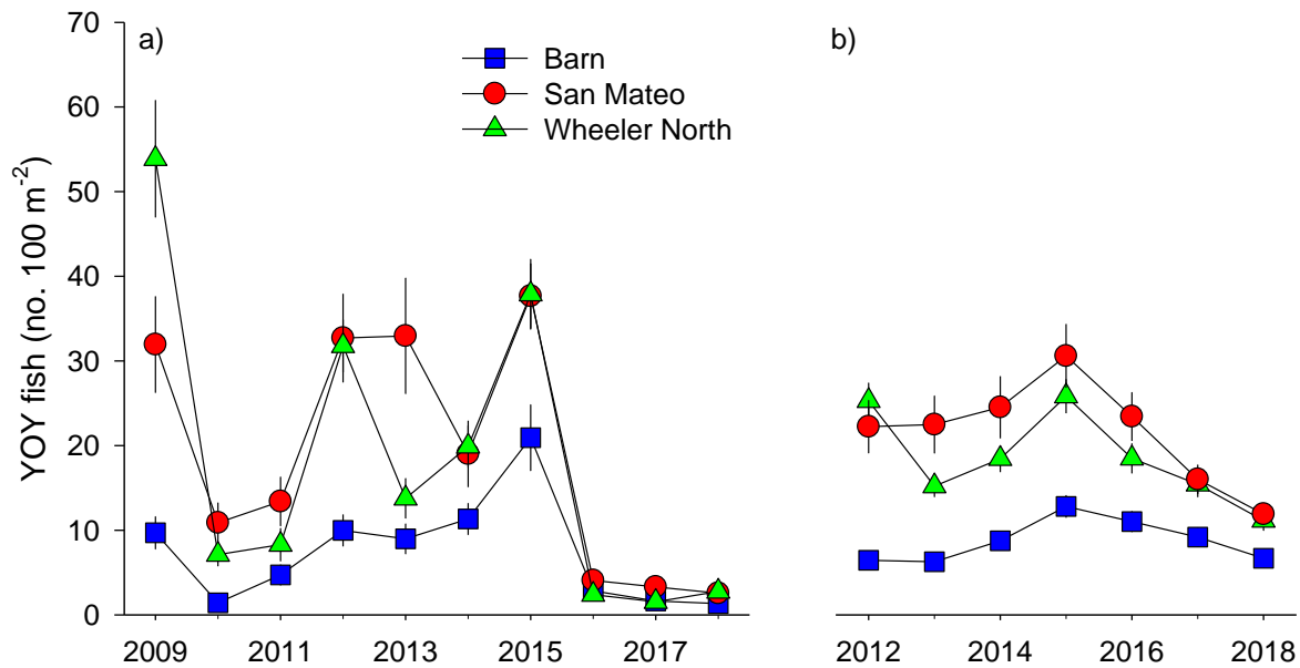
Figure 6.12. Mean density ( \pm 1 standard error) of young-of year fish at Wheeler North Reef, San Mateo and Barn (a) annual values for 2009 – 2018 and (b) 4-year running average.
