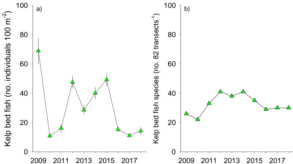
Figure 5.2.18. (a) Mean density ( \pm 1 standard error) and (b) total number of species of kelp bed fish near the bottom at Wheeler North Reef from 2009 – 2018.
