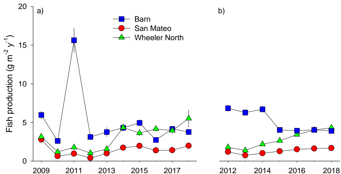
Figure 6.114. Mean fish production ( \pm 1 standard error) at Wheeler North Reef, San Mateo and Barn (a) annual values from 2009 – 2018 and (b) 4-year running average.
