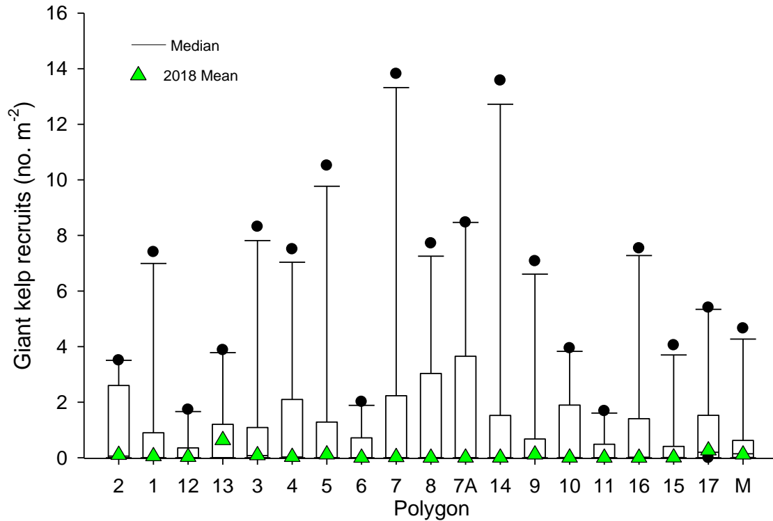
Figure 5.2.2. Mean densities of newly recruited giant kelp plants ( Macrocystis pyrifera ) in the Phase 2 polygons of Wheeler North Reef from 2009 – 2018. Box boundaries indicate the 25 th and 75 th percentiles and the whiskers are the 10 th and 90 th percentile. Solid points represent the upper and lower range. Polygon numbers are ordered from south to north. M represents the twelve Phase 1 modules.
