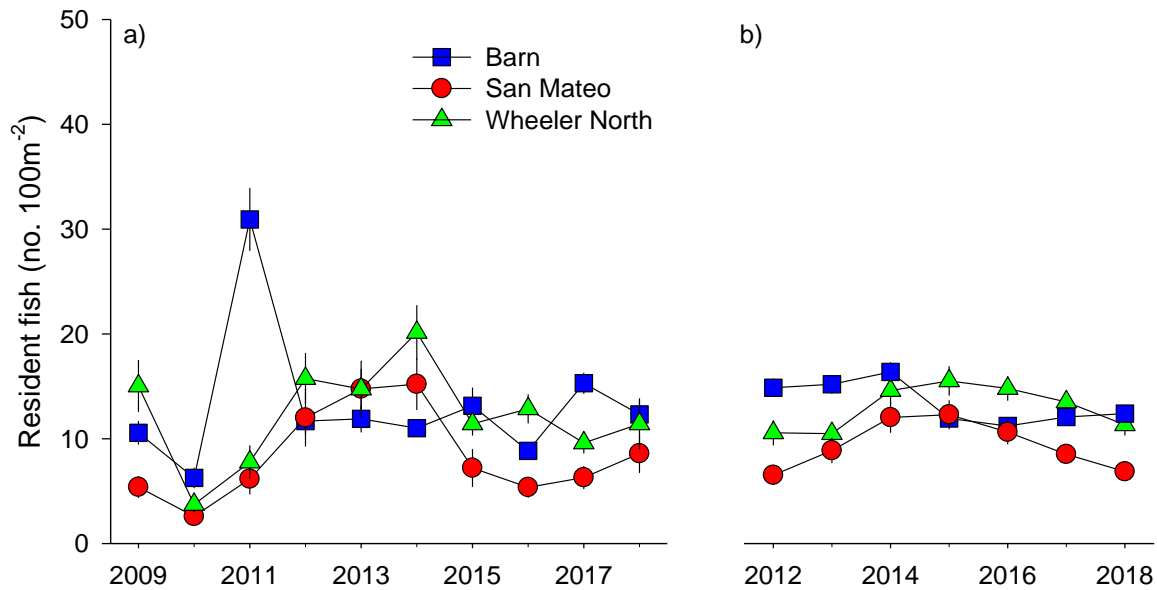
Figure 6.11. Mean density ( \pm 1 standard error) of resident fish at Wheeler North Reef, San Mateo and Barn (a) annual values for 2009 – 2018 and (b) 4-year running average.
