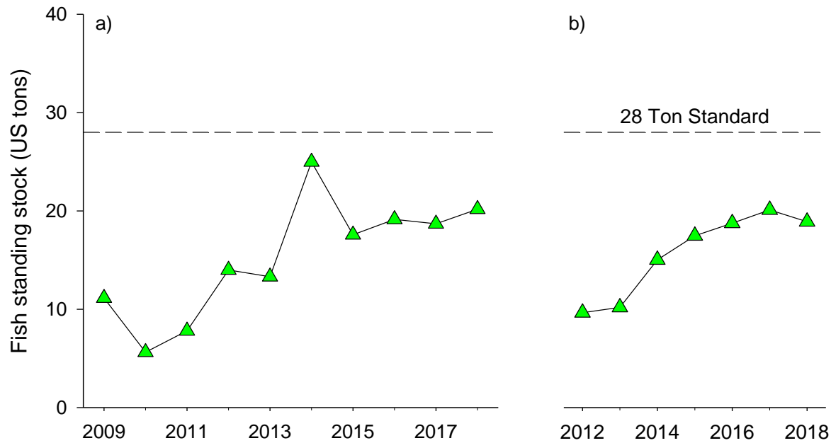
Figure 6.3. Estimated standing stock of fish at Wheeler North Reef (a) annual values for 2009 – 2018 and (b) 4-year running average.
