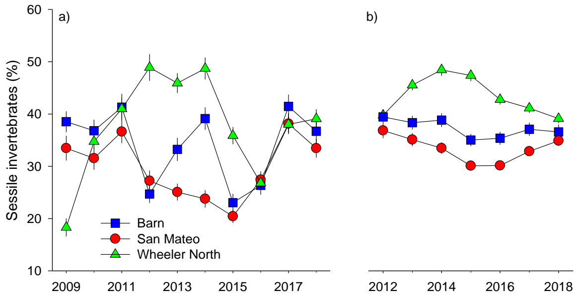
Figure 6.8. Mean percent cover ( \pm 1 standard error) of sessile invertebrates at Wheeler North Reef, San Mateo and Barn (a) annual values for 2009 – 2018 and (b) 4-year running average.
