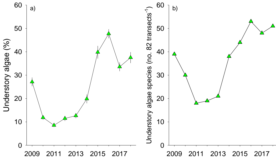
Figure 5.2.8. (a) Mean percent cover ( \pm 1 standard error) and (b) total number of species of understory algae at Wheeler North Reef from 2009 – 2018.
