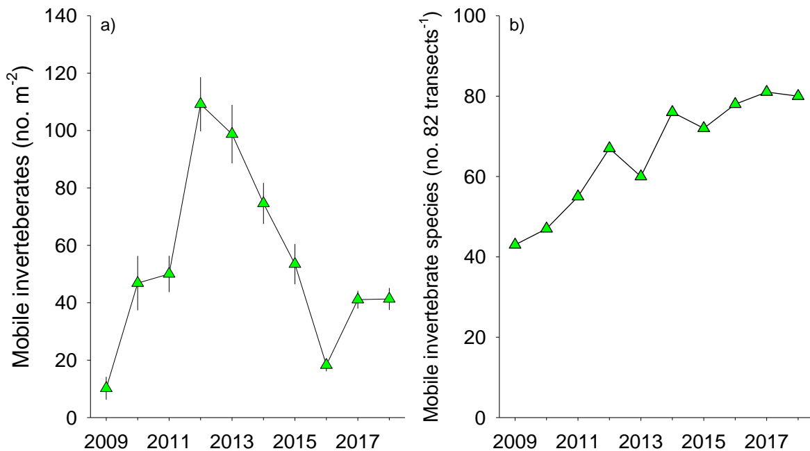
Figure 5.2.15. (a) Mean density ( \pm 1 standard error) and (b) total number of species of mobile invertebrates at Wheeler North Reef from 2009 – 2018.
