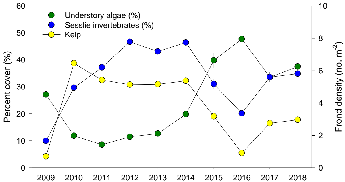
Figure 5.2.12. Comparison of mean percent cover ( \pm 1 standard error) of understory algae (green) and sessile invertebrates (blue) on left axis and mean density ( \pm 1 standard error) of adult giant kelp (yellow) on the right axis at Wheeler North Reef from 2009 – 2018.
