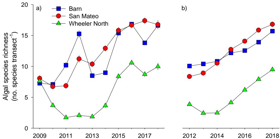
Figure 6.7. Mean species density ( \pm 1 standard error) of understory algae at Wheeler North Reef, San Mateo and Barn (a) annual values for 2009 – 2018 and (b) 4-year running average.
