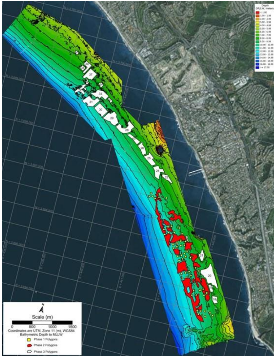
Figure 7.4.1. Map showing the location of the existing Phase I modules, Phase II polygons and the expanded remediation reef (Phase III polygons).
