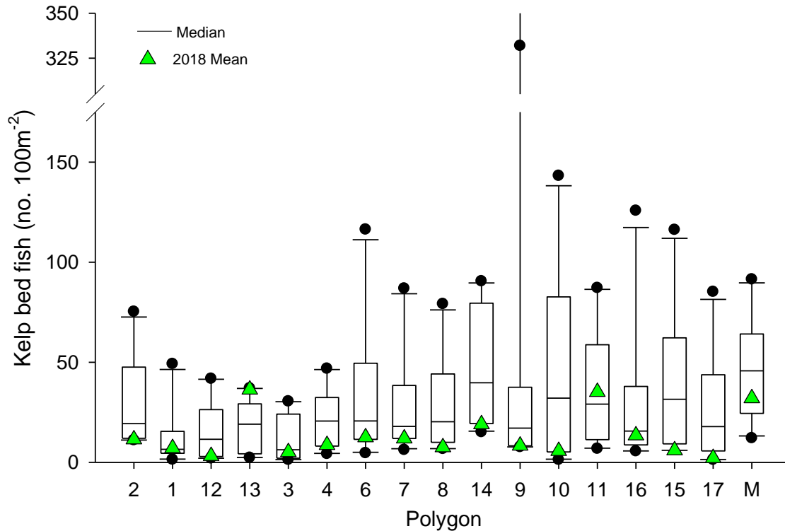
Figure 5.2.19. Mean densities of kelp bed fish in the Phase 2 polygons of Wheeler North Reef from 2009 – 2018. Box boundaries indicate the 25 th and 75 th percentiles and the whiskers indicate the 10 th and 90 th percentile. Solid points represent the upper and lower range. Polygon numbers are ordered from south to north. M represents the twelve Phase 1 modules.
