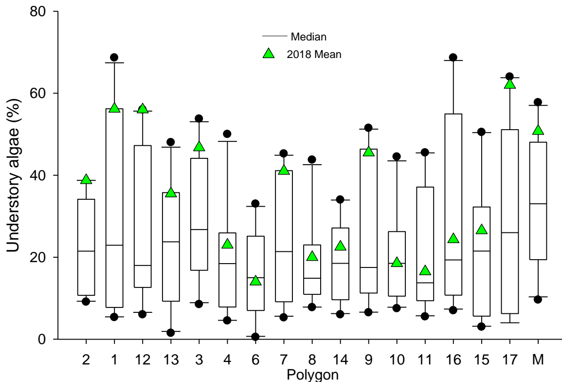
Figure 5.2.9. Mean percent cover of understory algae in the Phase 2 polygons of Wheeler North Reef from 2009 – 2018. Box boundaries indicate the 25 th and 75 th percentiles and the whiskers indicate the 10 th and 90 th percentile. Solid points represent the upper and lower range. Polygon numbers are ordered from south to north. M represents the twelve Phase 1 modules.
