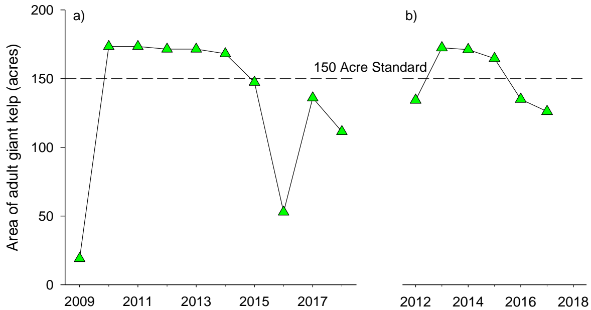
Figure 6.2. The number of acres of medium to high density adult kelp at Wheeler North Reef (a) annual values for 2009 – 2018 and (b) 4-year running average.
