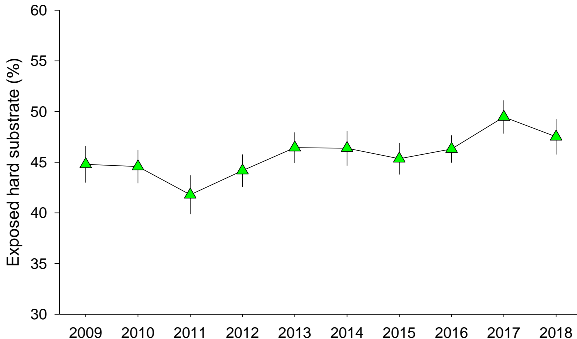
Figure 5.1.1. Mean percent cover ( \pm standard error) of exposed hard substrate at Wheeler North Reef from 2009 – 2018.
