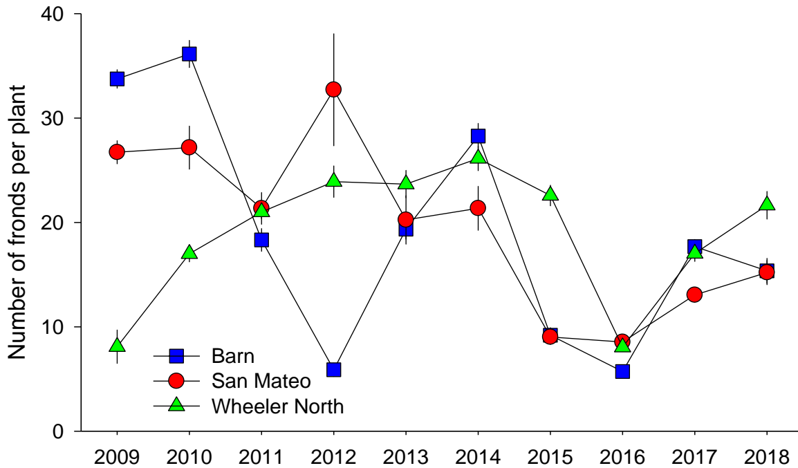
Figure 5.2.5. Mean number ( \pm 1 standard error) of fronds per Macrocyctis plant at Wheeler North Reef, Barn and San Mateo from 2009 – 2018.
