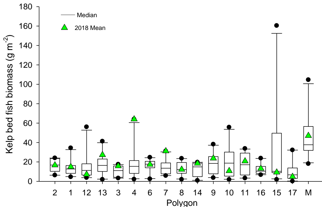
Figure 5.2.23. Mean biomass densities of kelp bed fish within 2 m of the bottom in the Phase 2 polygons of Wheeler North Reef from 2009 – 2018. Box boundaries indicate the 25th and 75th percentiles and the whiskers indicate the 10th and 90th percentile. Solid points represent the upper and lower range. Polygon numbers are ordered from south to north. M represents the 12 Phase 1 modules.
