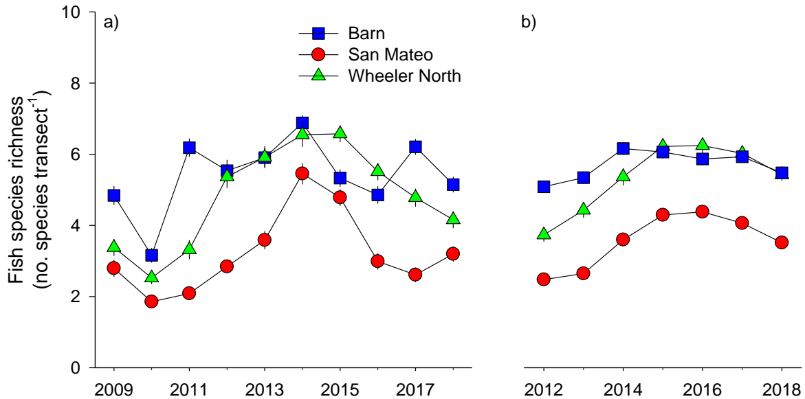
Figure 6.13. Mean species density ( \pm 1 standard error) of fish at Wheeler North Reef, San Mateo and Barn (a) annual values for 2009 – 2018 and (b) 4-year running average.
