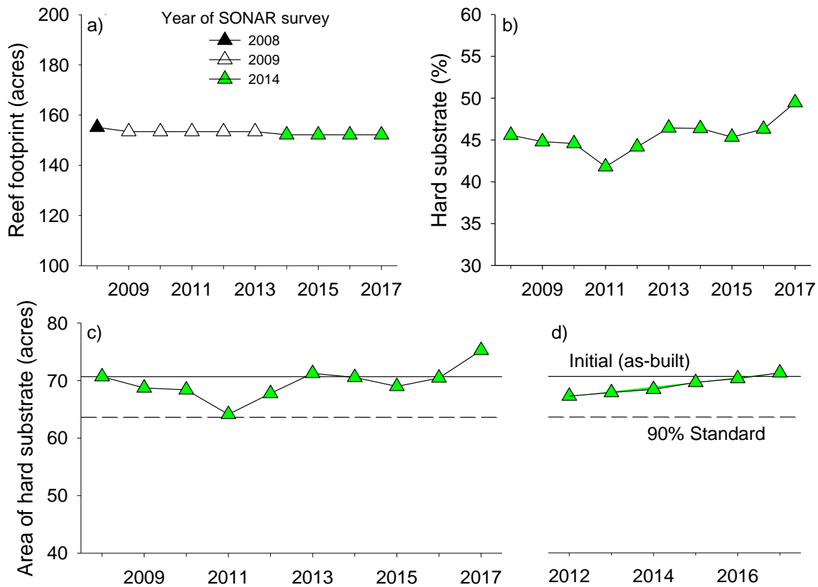
Figure 6.1 Variables used to calculate exposed hard substrate. (a) Reef footprint area, (b) Percent cover of hard substrate, (c) Area of exposed hard substrate and (d) 4-year running average of the area of exposed hard substrate.
