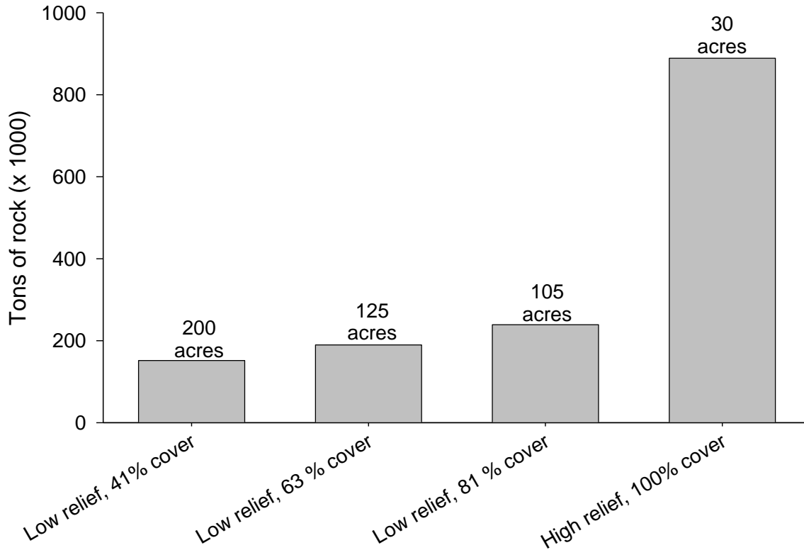
Figure 7.4.1 The tonnage of rock needed to construct the four different reef designs shown in Table 7.4.1, which when added to the existing Wheeler North Reef are expected to support a fish standing stock of 28 tons with 95% level confidence. Numbers above each bar are the numbers of acres of additional reef needed for each reef design as per Table 7.4.1.
