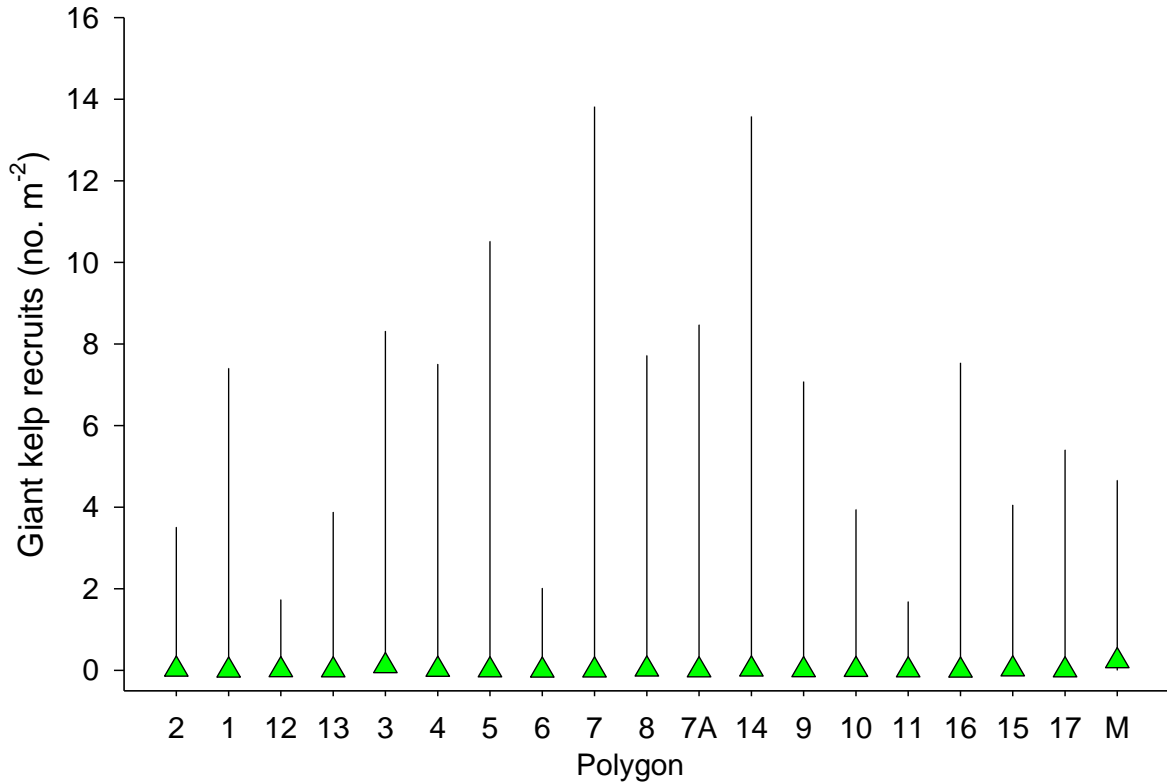
Figure 5.2.2 Mean density of newly recruited giant kelp plants ( Macrocystis pyrifera ) at Wheeler North Reef in 2017. Vertical lines represent the range of values observed from 2009 - 2017, with the largest values occurring in 2015 in most polygons. Polygon numbers are ordered from south to north. M is the mean of the twelve Phase 1 modules.
