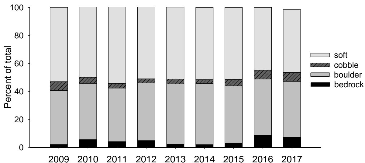
Figure 5.1.3 Distribution of substrate types on Wheeler North Reef from 2009 - 2017.
